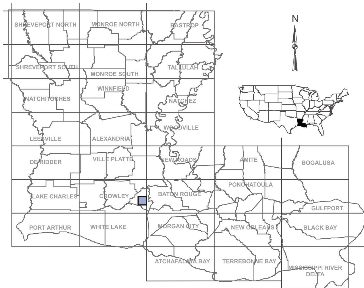
1. Location of Lafayette 7.5-minute quadrangle, southeastern Louisiana.
